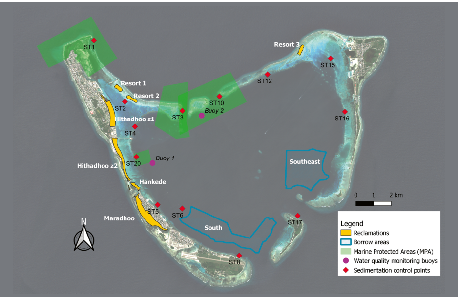
FIGURE 2 General outline of the reclamation project in Addu City.
