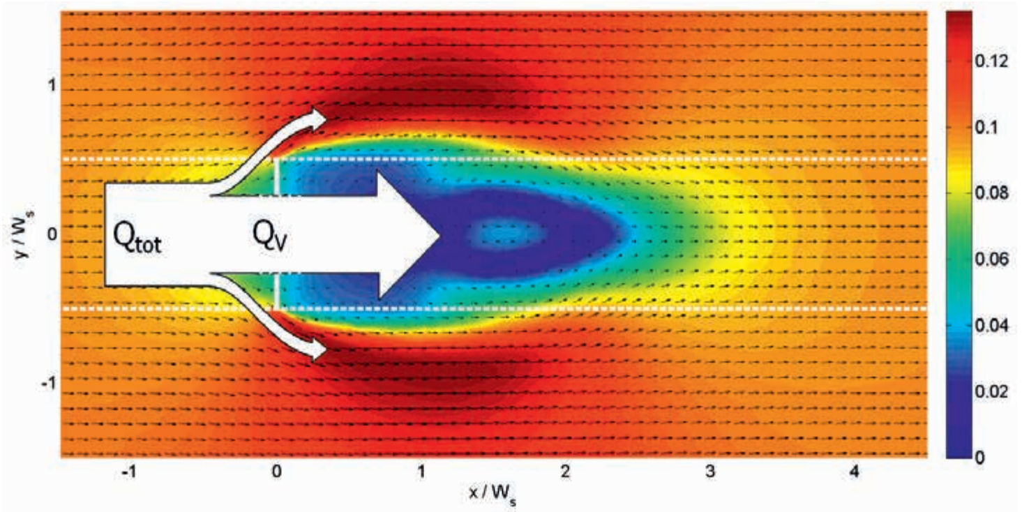
Figure 7. Example of a model current simulation with silt screen. The colours and vector arrows represent magnitude and direction of the depth-averaged flow velocity.
