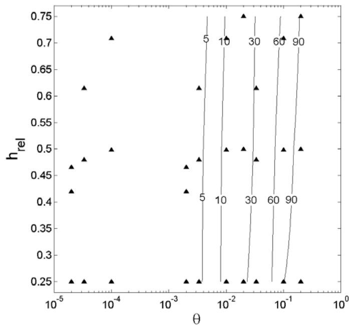
Figure 5. Inflow effectiveness [%] evaluated at 6h downstream of the silt screen, as a function of the velocity ratio and relative screen height, for a uniform upstream SSC profile.
