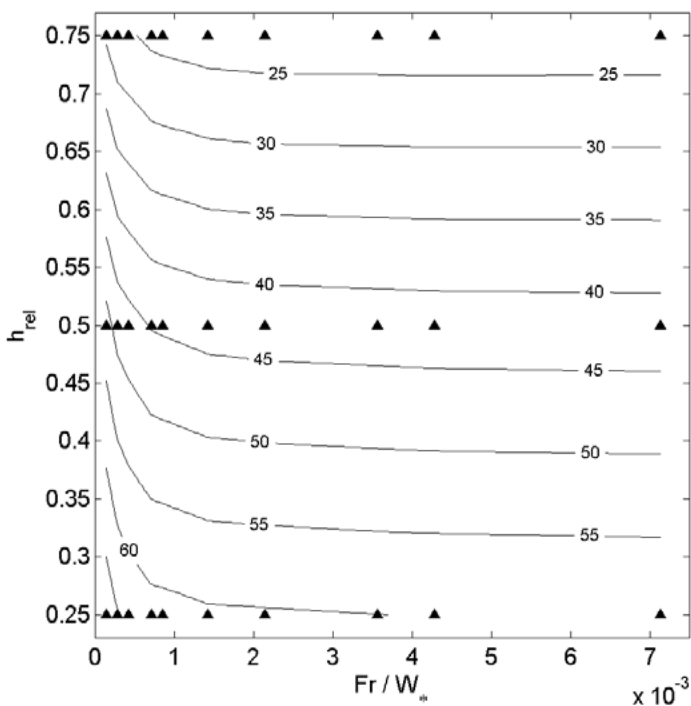
Figure 8. Relative discharge [%] as a function of relative screen height and Froude number over relative screen width.
