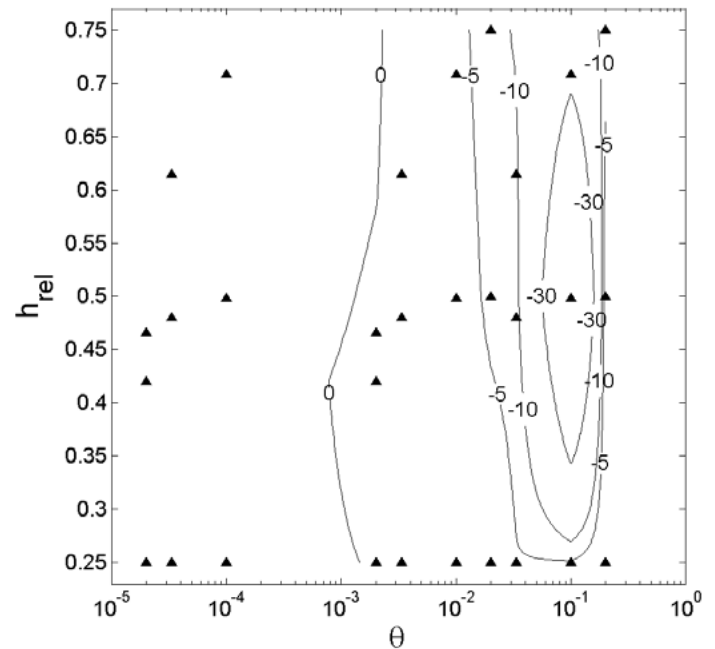
Figure 6. Reference effectiveness [%] evaluated at 6h downstream of the silt screen, as a function of the velocity ratio and relative screen height, for a uniform upstream SSC profile.
