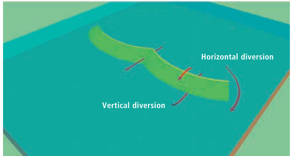
Figure 2. Current flows around a hanging silt screen: Main components are the flow under the screen (vertical diversion) and the flow around the screen's side edges (horizontal diversion).
