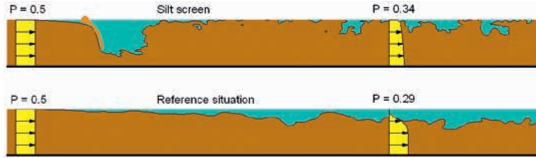
Figure 3. Example of application of percentage of reduction of P achieved by the screen. The yellow profiles represent values of C_* , whereas the value of C_* z_* , integrated over z_* , is given above each profile. In this situation, E_{in} = 32\% and E_{ref} = -10\% .
