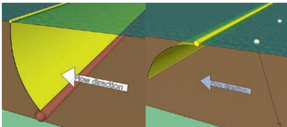
Figure 1. Standing (left) and hanging (right) silt screens.
