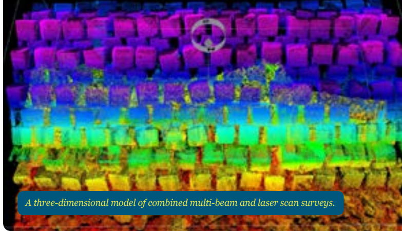
The visualisation of a multi-beam echo-sounding.
